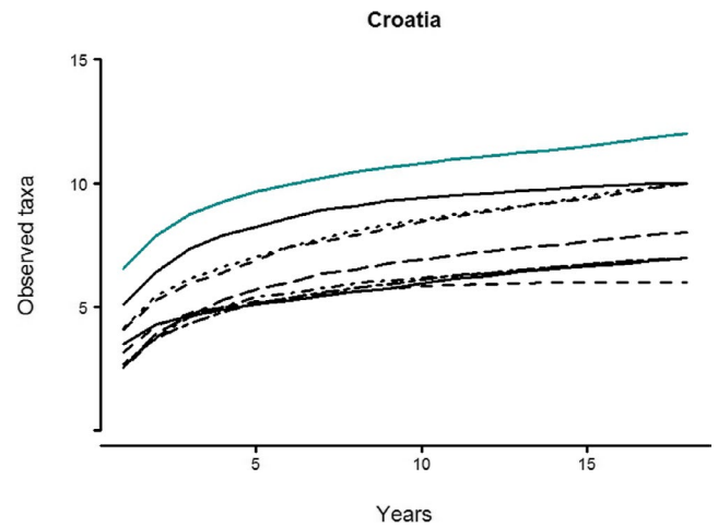
FIGURE 1 Accumulation of observed insect taxa during 18 years of sampling (2001–2018) in eight Croatian Forestry units (black curves) and in all Forestry units combined (upper, blue curve)
