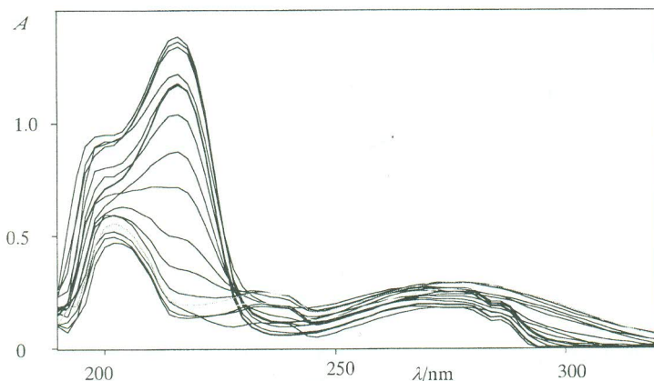
Figure 2. Ultraviolet absorption spectra of indolyl-3-acetic acid ( c = 4.0 \cdot 10^{-5} mol/dm 3 ) as function of perchloric acid concentration. Solvent (top to bottom, at position of \lambda = 220 nm) perchloric acid 1.0; 2.0; 3.0; 3.5; 4.0; 4.5; 5.0; 5.5; 6.0; 6.5; 7.0; 7.5; 8.0; 8.5; 9.0; 9.5 and 10.0 mol/dm 3 ).
