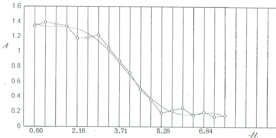
Figure 3. Effect of acidity function on absorbance at 216 nm of indole.
