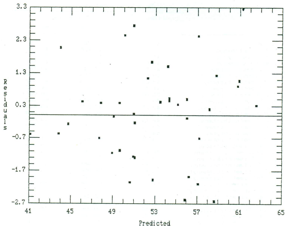
Figure 3. Plot of residuals versus calculated retention times using eq. 7.
